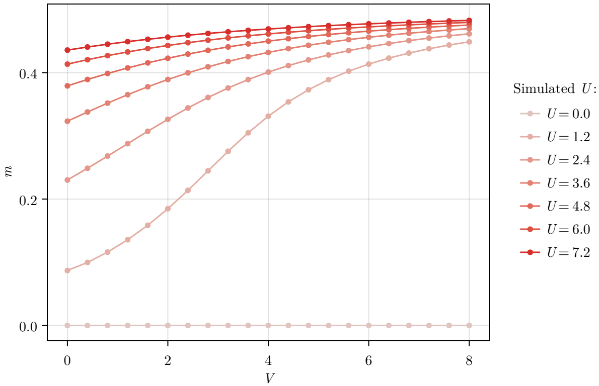
Magnetization ( t = 1.0 , L = 256 , \delta = 0.0 , \beta = 100.0 )
